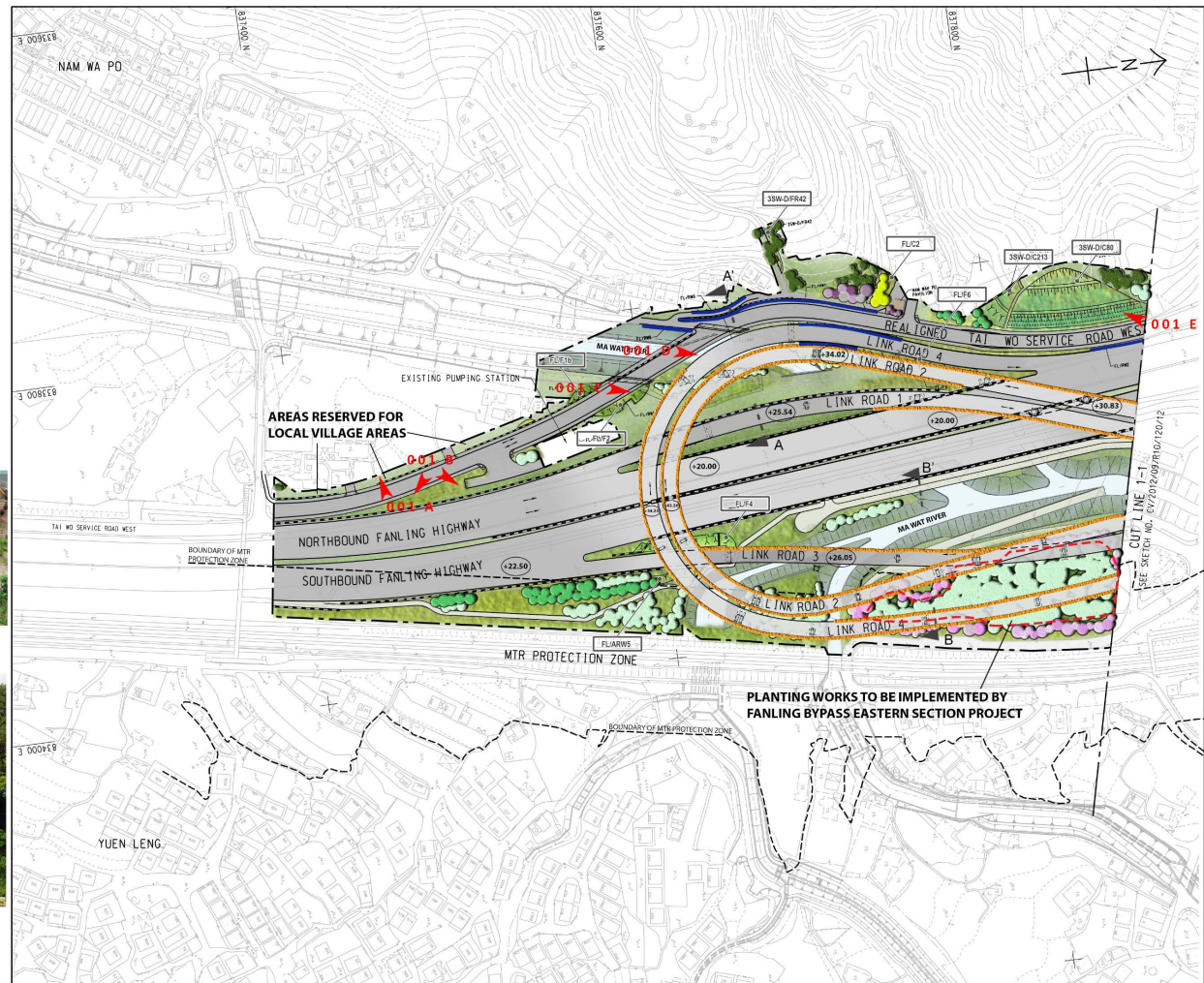
Shrubs and/or Groundcover Planting on Slope (OM10)
