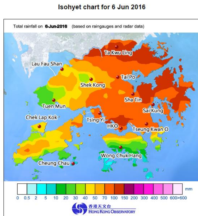
Figure 2 Rainfall distribution on 6 June 2016
