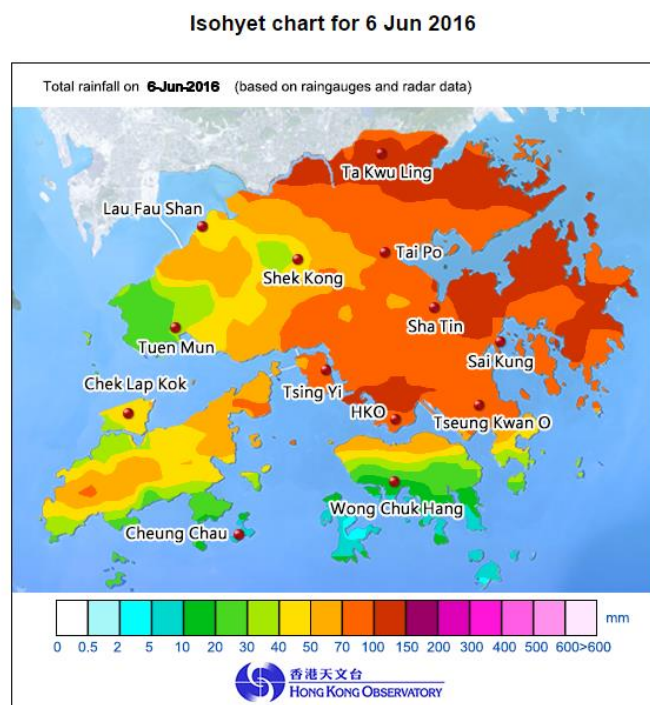
Figure 2 Rainfall distribution on 6 June 2016
