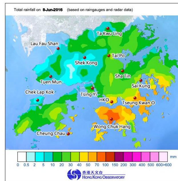
Figure 4: Rainfall distribution on 8 June 2016
